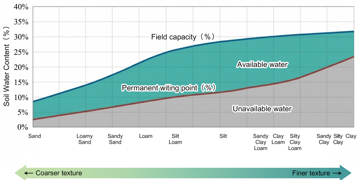
Figure 3. Reference chart for available soil water
