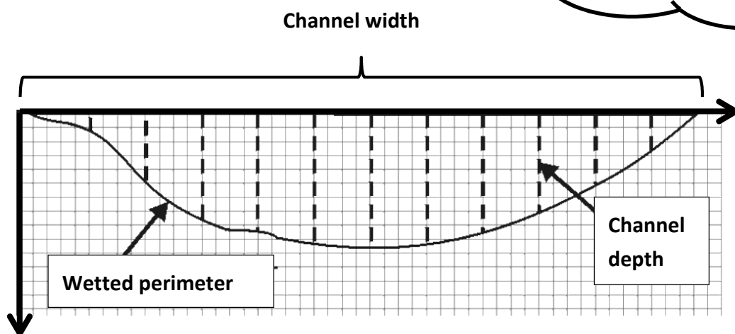
↑ Figure 2: Cross-section of a channel.
